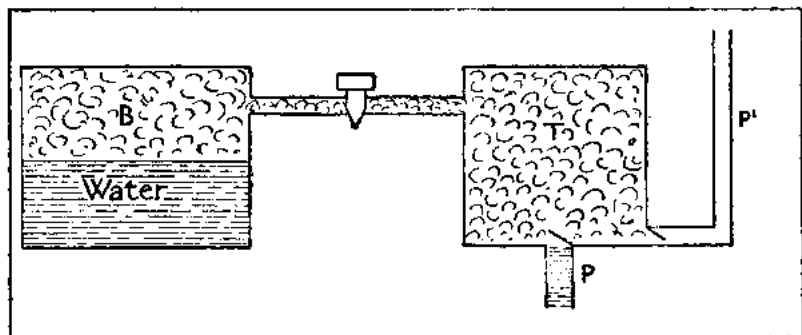
DIAGRAM OF SAVERY'S ENGINE.
