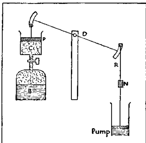
DIAGRAM OF NEWCOMEN'S ENGINE.
